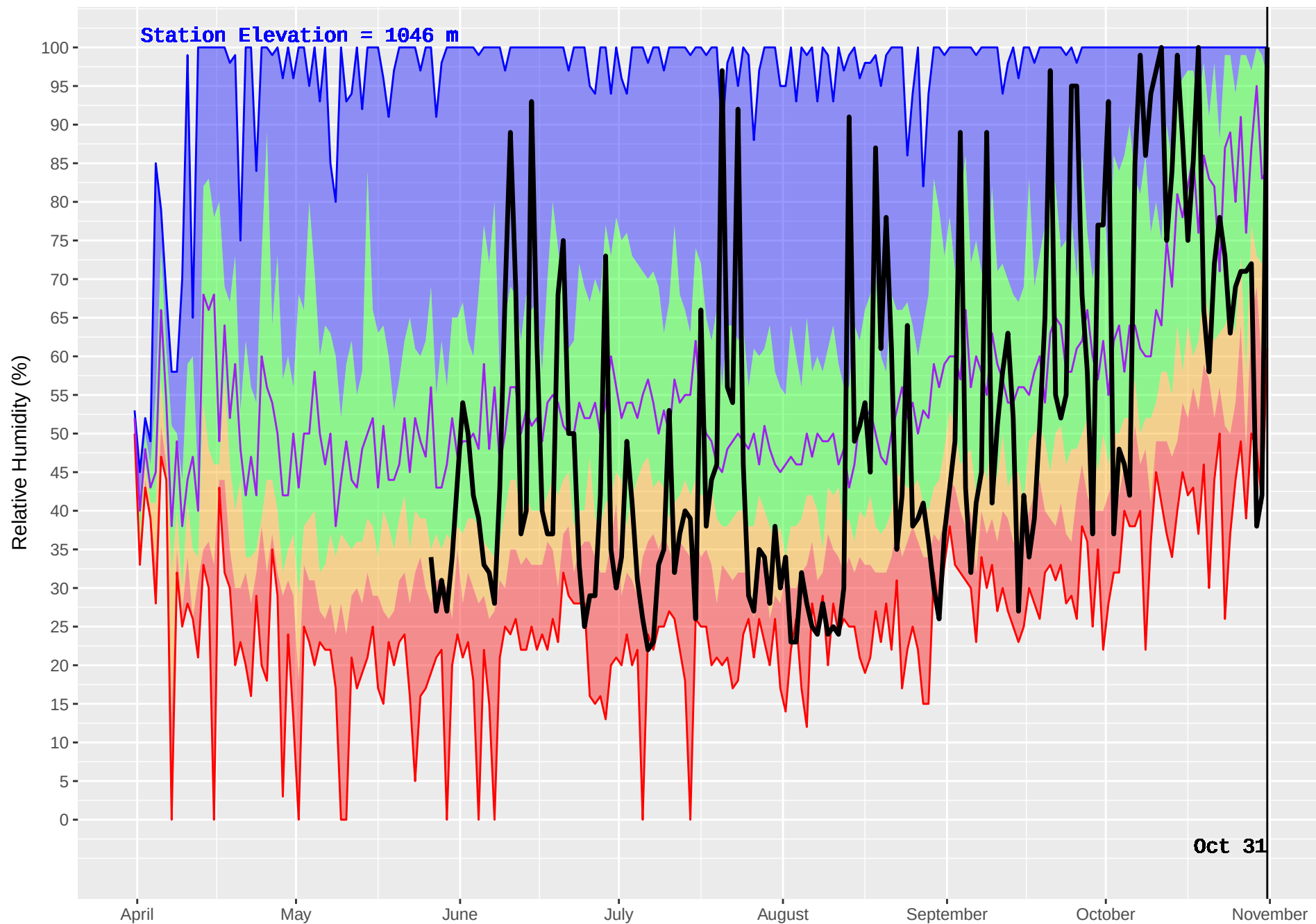
LIKELY RS (255) : Historical (1970–2016) and Current (2017) Noon Relative Humidity
