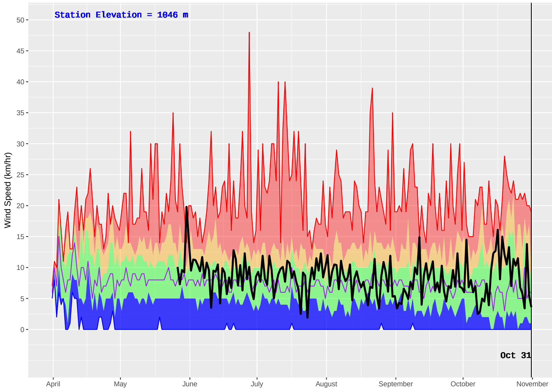
LIKELY RS (255) : Historical (1970–2016) and Current (2017) Noon Wind Speed
